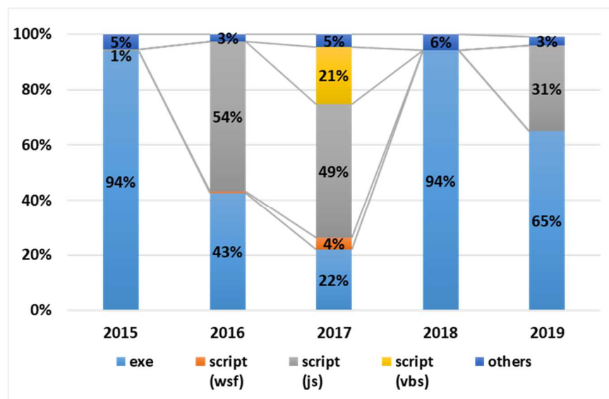
Figure 7 [Composition of compressed attachments to spear phishing emails]
