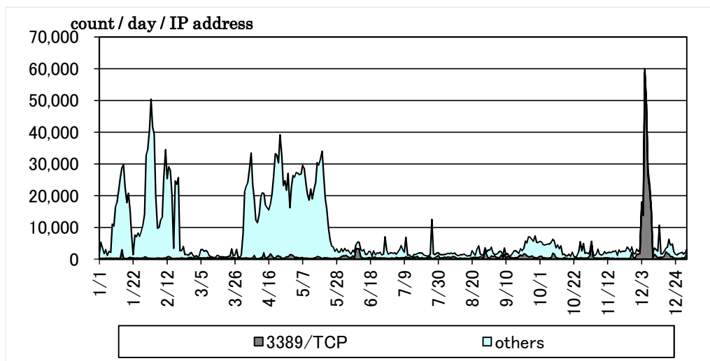
Figure 3 [Connection attempts to a wide range of ports for targeting the Remote Desktop services]
